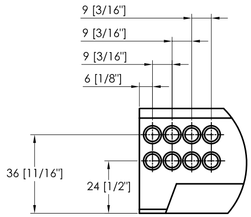
DETAIL B SCALE 1:2
