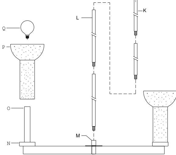
Install at least 1pcs 12" tube ( L ) as you assemble
