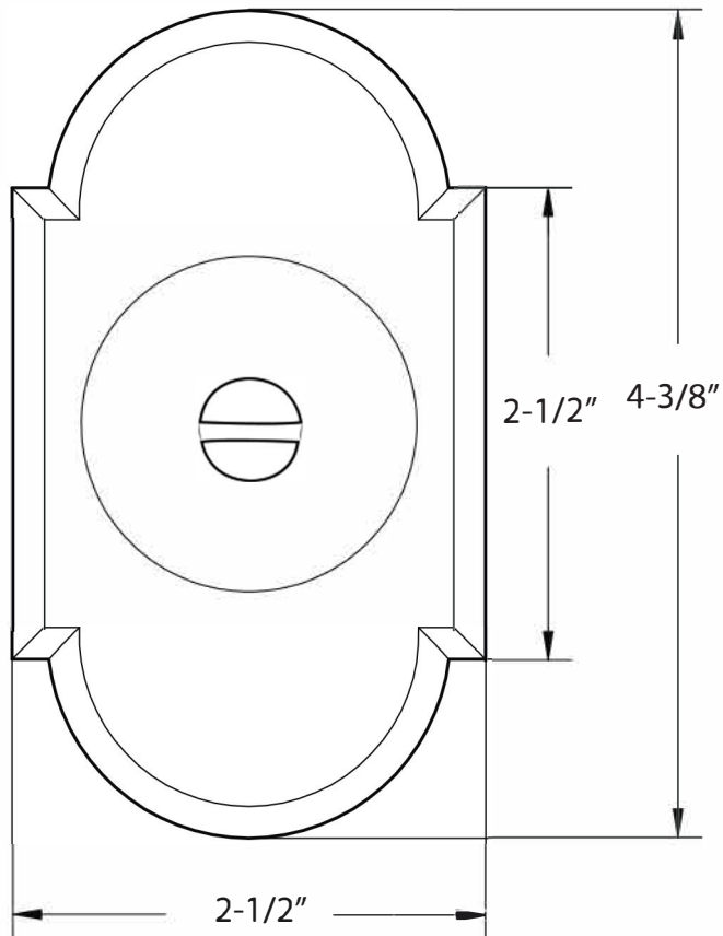
#8 TUBULAR POCKET PRIVACY, OUTSIDE TRIM
