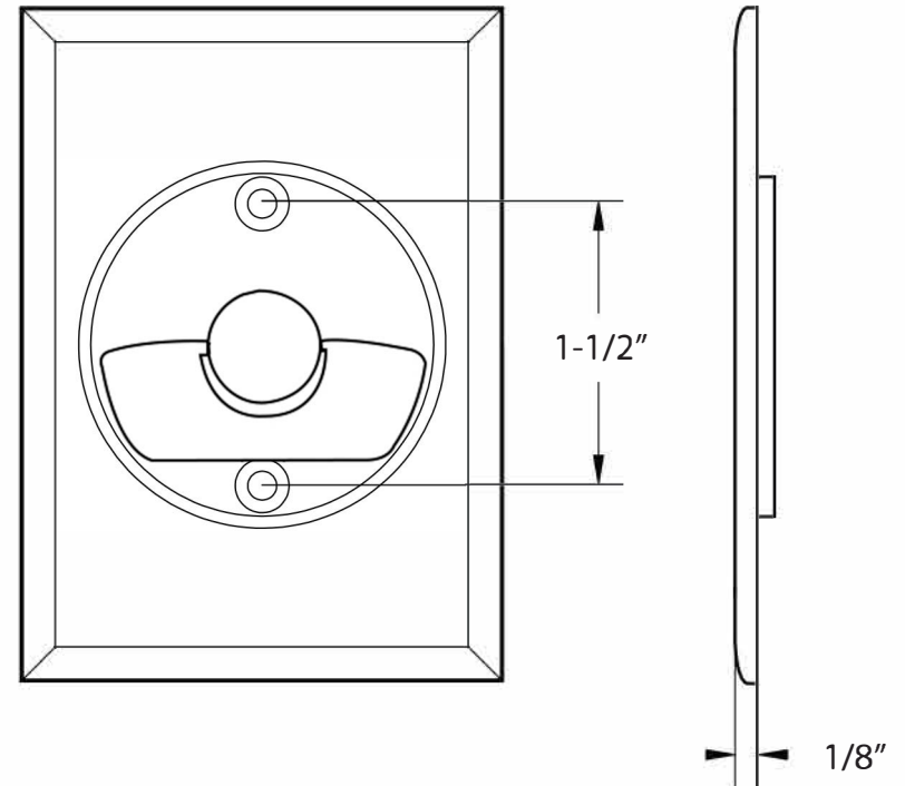
RECTANGULAR TUBULAR POCKET PRIVACY, INSIDE TRIM
