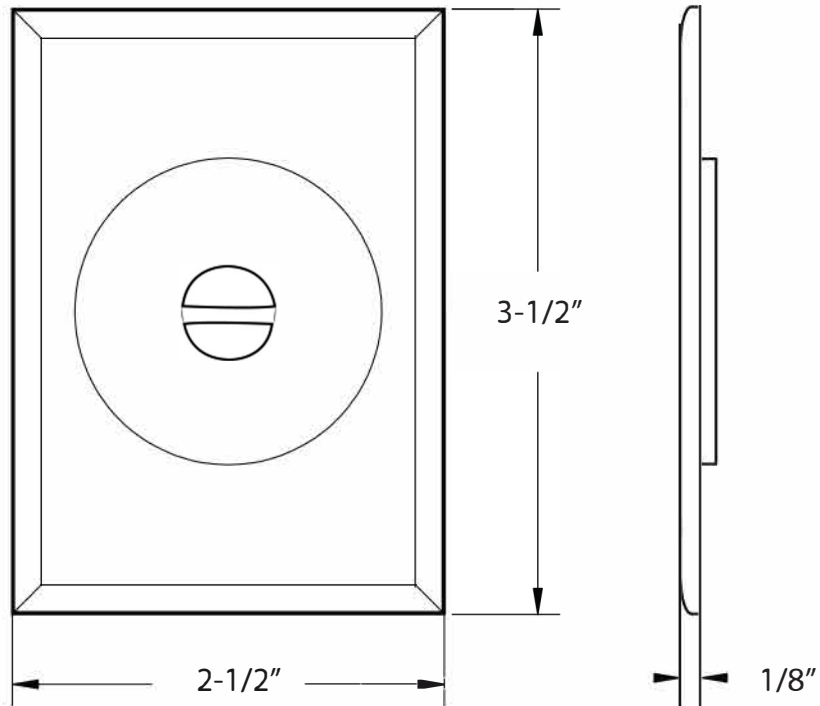
RECTANGULAR TUBULAR POCKET PRIVACY, OUTSIDE TRIM
