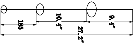
CRS39853PCK*2PCS L: 27.17"
