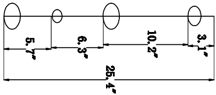
CRS39853PCD*3PCS L: 25.39"
