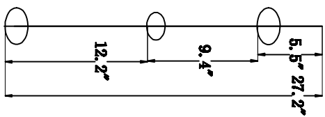
CRS39853PCG*4PCS L: 27.17"
