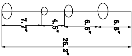
CRS39853PCL*2PCS L: 25.2"
