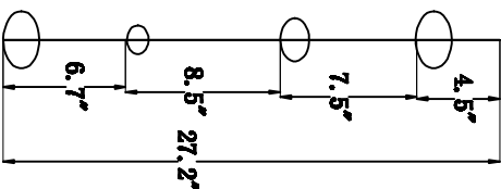
CRS39853PCN*1PC L: 27.17"
