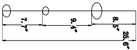
CRS39853PCF*4PCS L: 25.59"
