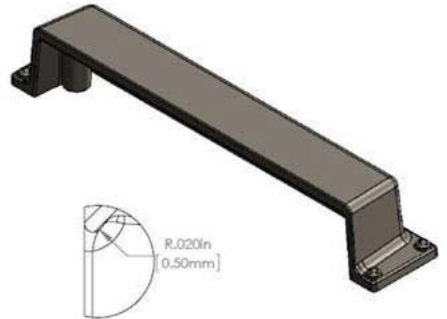
DETAIL AD SCALE 4:1
