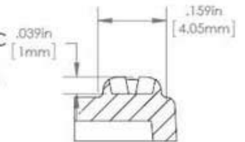
SECTION AC-AC SCALE 4:1
